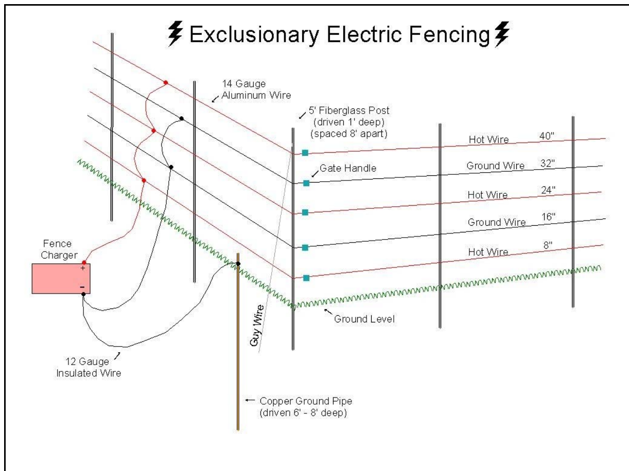
Figure 1. Diagram of properly constructed electric fence to exclude bears.
